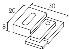
223999 Supporto a soffitto Ceiling bracket Support à plafond
