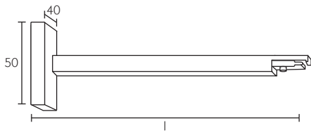
2233-- Supporto Bracket Support
