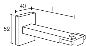
2232-- Adele 353-- Clara Supporto
